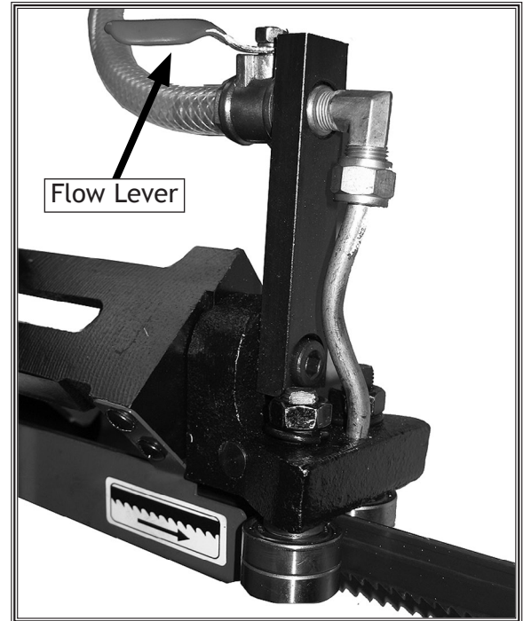
Figure 35. Lubricator flow control lever.
